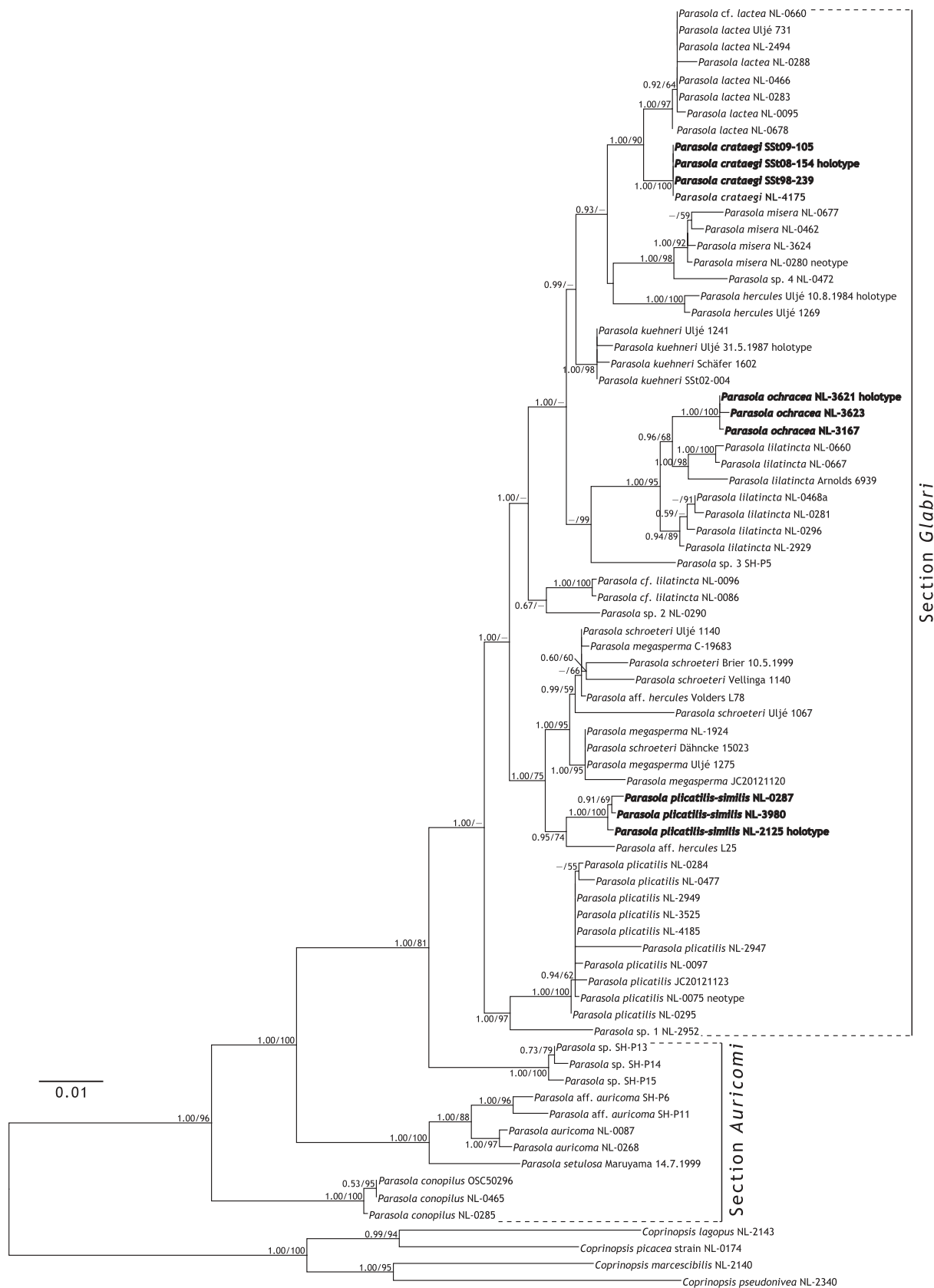
Figure 1. The 50% majority rule phylogram constructed from post-burn-in trees of the Bayesian analyses of 28S+ITS data. Numbers on the branches represent Bayesian posterior probabilities followed by ML bootstrap values. An asterisk (*) indicates 100% bootstrap or 1.00 posterior probabilities, whereas a minus sign (-) indicates support values lower than 50% bootstrap or 0.70 posterior probability. Sequences of the newly described species highlighted in boldface. Bar indicates 0.01 expected change per site per branch.
